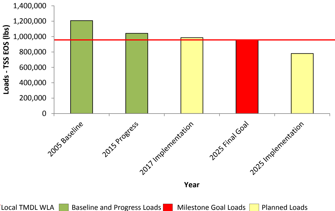
Figure 9: Progress and Planned Reductions in the Little Patuxent River Watershed
