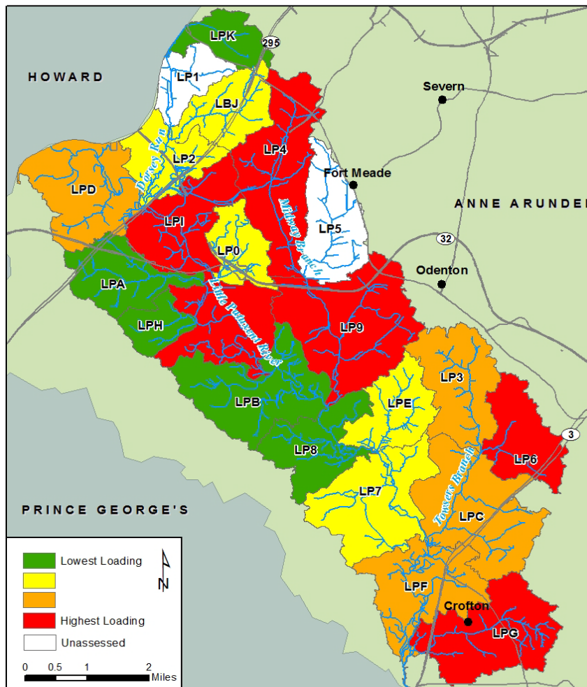
Figure 5: Total Suspended Solids Load from Runoff Based on Existing Conditions - Includes BMP Reductions (Anne Arundel County, 2014 Draft)
