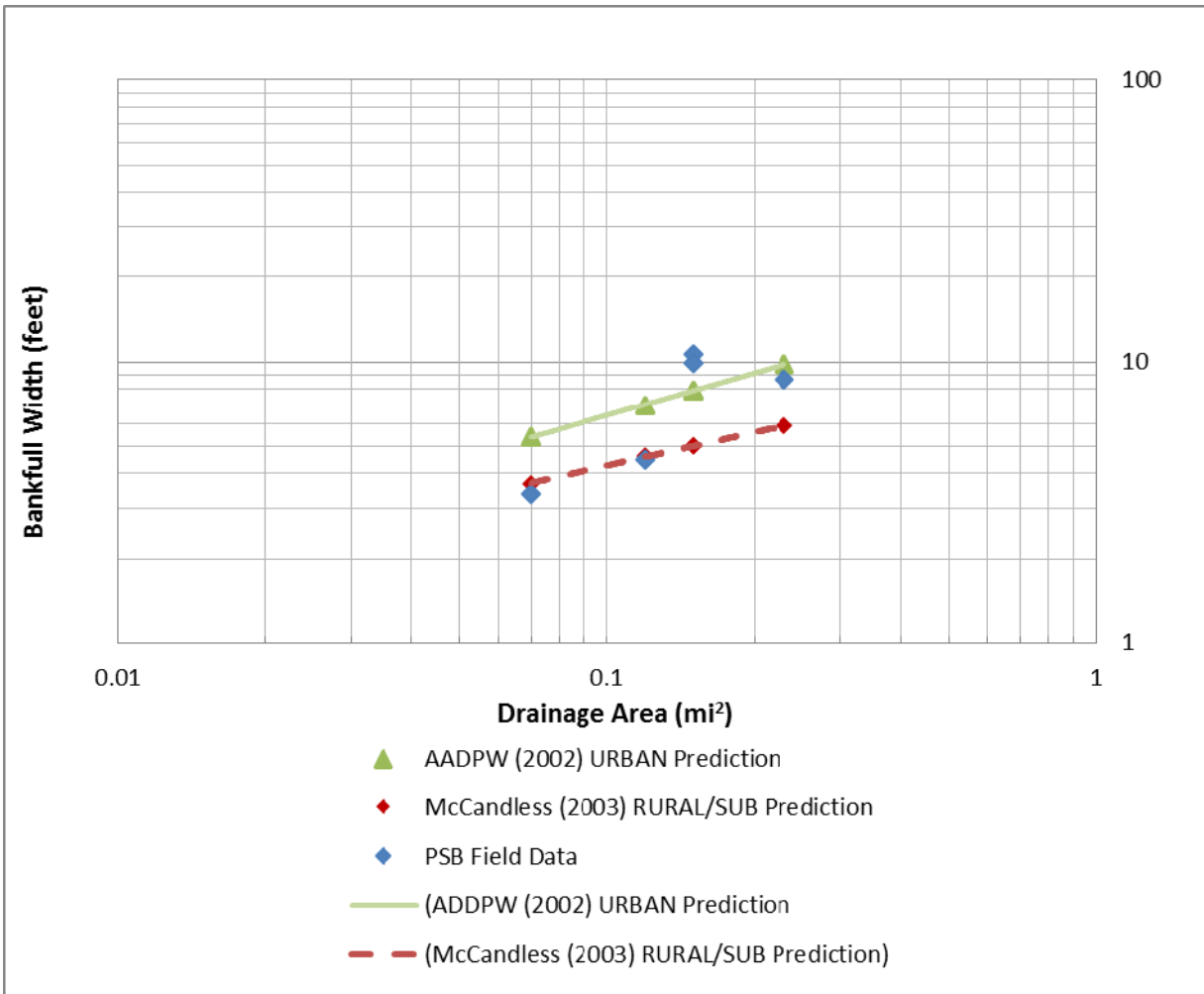
Figure 3-1. Comparison of the bankfull width drainage area relationship between Picture Spring Branch (PSB) 2015 field data and regional relationship curve data
