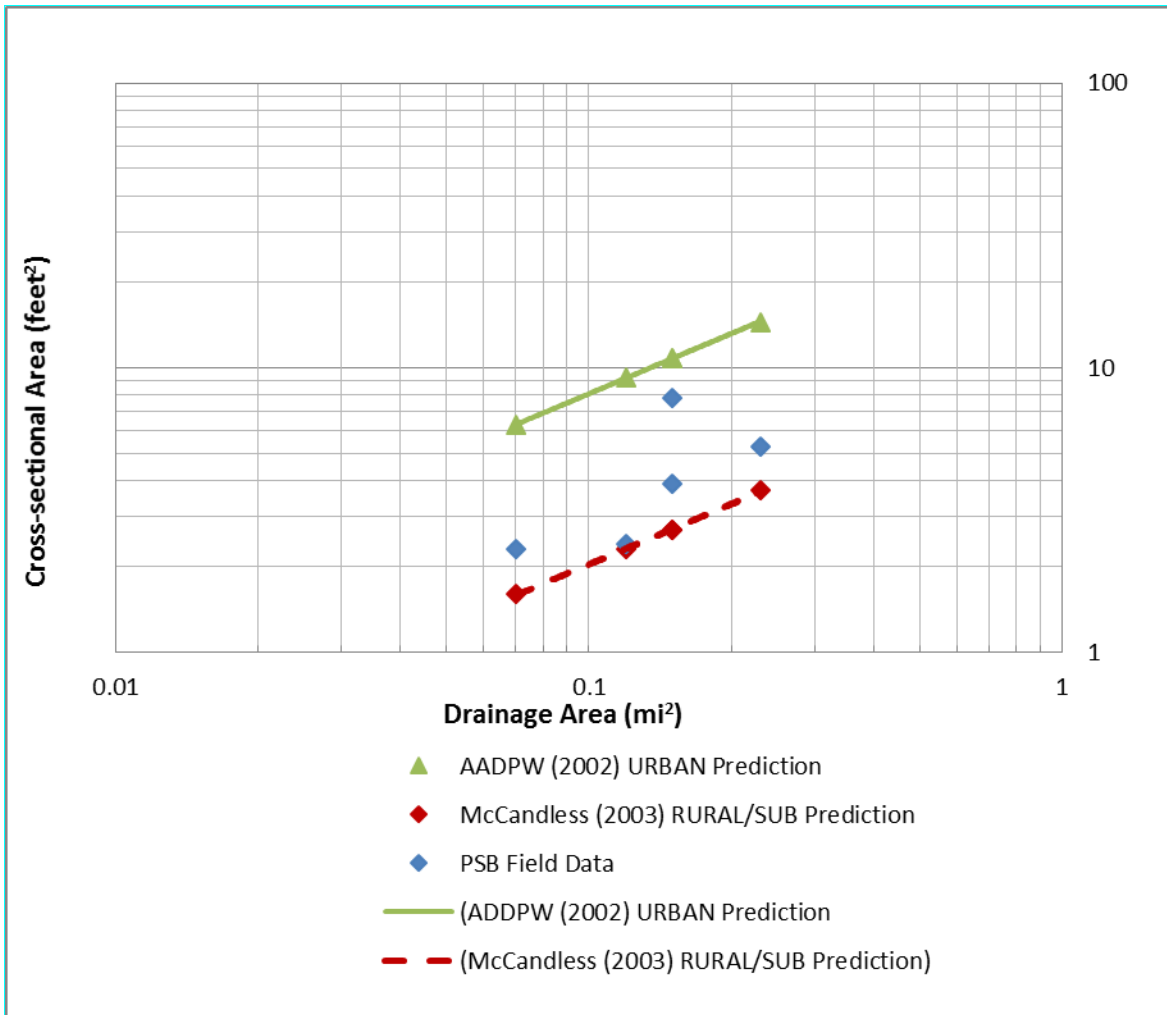
Figure 3-2. Comparison of the bankfull cross-sectional area drainage area relationship between Picture Spring Branch 2015 field data and regional relationship curve data
