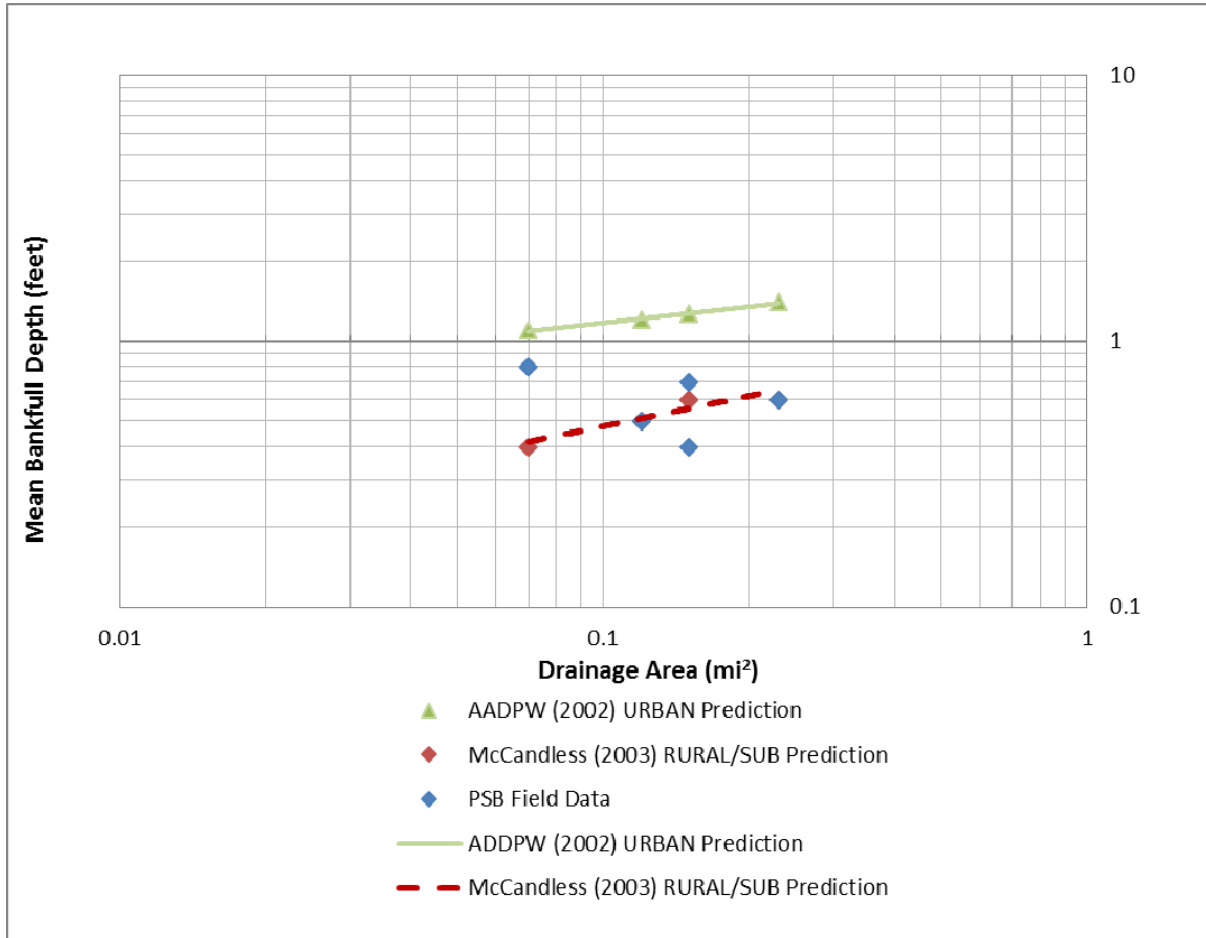
Figure 3-3. Comparison of the mean bankfull depth drainage area relationship between Picture Spring Branch 2015 field data and regional relationship curve data
